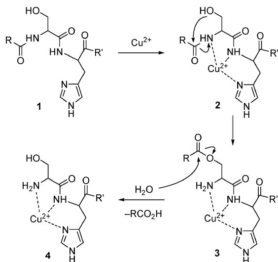
Scheme 1. Proposed mechanism for \text{Cu}^{2+} -assisted hydrolysis of a Xaa-Ser-His sequence.
