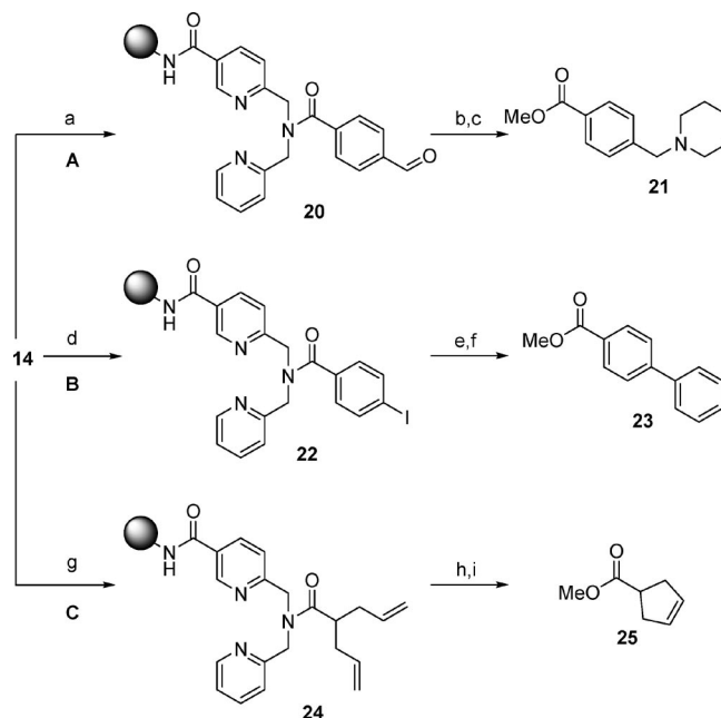
Scheme 7. Reactions on the bpa linker. Reagents and conditions: (a) 4-carboxybenzaldehyde (3.0 equiv.), TBTU (3.0 equiv.), DIPEA (12 equiv.), DMF, r.t., 12 h; (b) piperidine (10 equiv.), NaBH(OAc) 3 (10 equiv.), 1,2-DCE, r.t., 12 h; (c) Cu(OTf) 2 (1.0 equiv.), MeOH, r.t., 12 h, 49% over 5 steps; (d) 4-iodobenzoic acid (3.0 equiv.), TBTU (3.0 equiv.), DIPEA (12 equiv.), DMF, r.t., 12 h; (e) PhB(OH) 2 (5.0 equiv.), K 3 PO 4 (10 equiv.), Pd(PPh 3 ) 4 (10 mol-%), DMF, 90 °C, 12 h; (f) Cu(OTf) 2 (1.0 equiv.), MeOH, r.t., 12 h, 31% over 5 steps; (g) 2-allyl-4-pentenoic acid (3.0 equiv.), TBTU (3.0 equiv.), DIPEA (12 equiv.), DMF, r.t., 12 h; (h) Grubbs 2nd generation catalyst (5 mol-%), CH 2 Cl 2 , r.t., 24 h; (i) Cu(OTf) 2 (1.0 equiv.), MeOH, r.t., 12 h, 34% over 5 steps.
