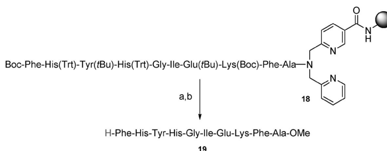
Scheme 6. Cleavage of decapeptide 19 . Reagents and conditions: (a) Cu(OTf) 2 (1.0 equiv.), MeOH; (b) TFA/CH 2 Cl 2 /iPr 3 SiH, 95:3:2.
