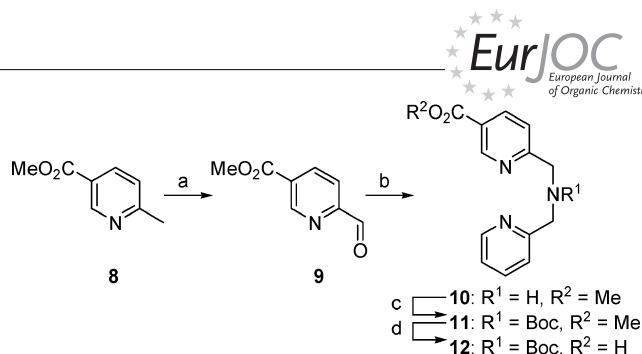
Scheme 3. Synthesis of Boc-protected bispicolylamide 12 . Reagents and conditions: (a) \text{I}_2 (1.0 equiv.), t\text{BuI} (0.4 equiv.), TFA (3.0 equiv.), DMSO, 120^\circ\text{C} , 3 h, 69%; (b) 2-picolylamine (1.0 equiv.), \text{NaBH}(\text{OAc})_3 (1.4 equiv.), 1,2-DCE, 1 h; (c) \text{Boc}_2\text{O} (1.2 equiv.), \text{NEt}_3 (1.4 equiv.), \text{CH}_2\text{Cl}_2 , 0^\circ\text{C} \rightarrow \text{r.t.} , 2 h, 69% over 2 steps; (d) NaOH (1.1 equiv.), MeOH/ \text{H}_2\text{O} , reflux, 2 h, >98%.
