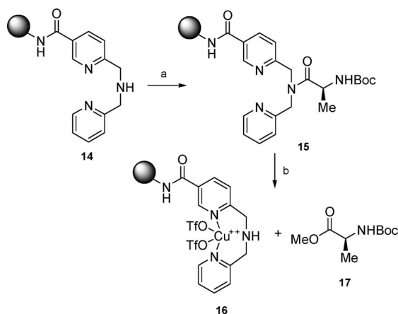
Scheme 5. Coupling of Boc-Ala-OH and Cu 2+ -assisted cleavage to methyl ester 17 . Reagents and conditions: (a) Boc-Ala-OH (3.0 equiv.), TBTU (3.0 equiv.), DIPEA (12 equiv.), DMF, r.t., 12 h; (b) Cu(OTf) 2 (1.0 equiv.), MeOH, r.t., 12 h, 50% over 4 steps.
