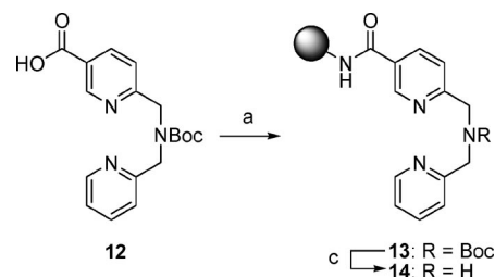
Scheme 4. Coupling of 12 to the solid support and cleavage of the Boc group. Reagents and conditions: (a) HypoGel-400- \text{NH}_2 , DMF, 10 min; then 12 (1.5 equiv.), TBTU (1.5 equiv.), DIPEA (6.0 equiv.), DMF, r.t., 12 h; (b) i\text{Pr}_3\text{SiH} (3.0 equiv.), \text{CH}_2\text{Cl}_2/\text{TFA} (1:1), 0^\circ\text{C} \rightarrow \text{r.t.} , 4 h.
