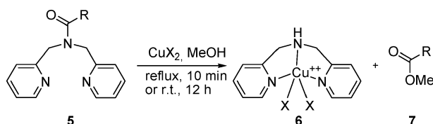
Scheme 2. \text{Cu}^{2+} -assisted hydrolysis of bispicolylamides; X = Cl, OTf, \text{ClO}_4 .
